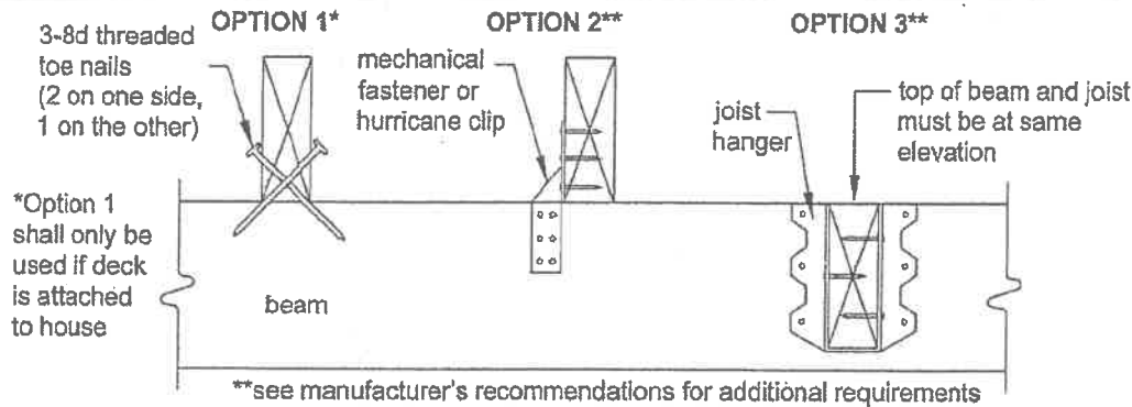
Figure 6: Joist-to-Beam Detail
