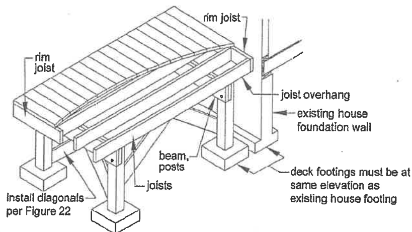
Figure 21. Free-Standing Deck
